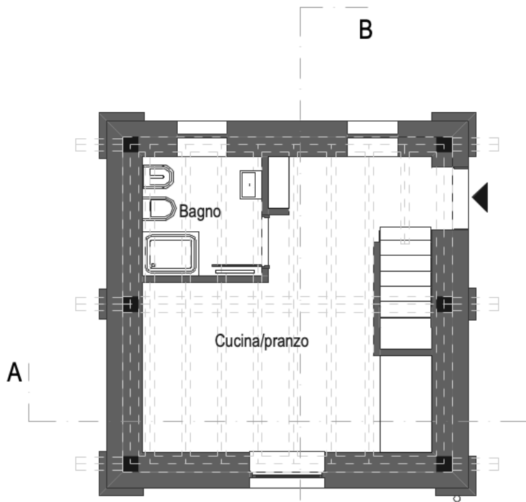
PIANO TERRA
