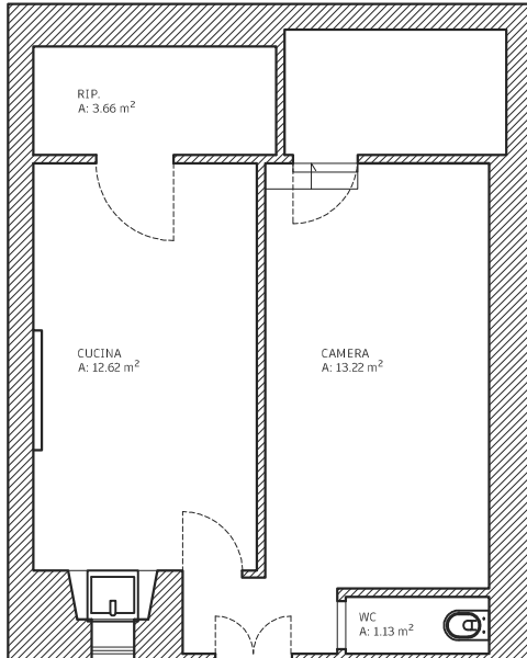
PIANO TERRA
